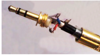
Figure 2-11 Two-Channel Wiring
