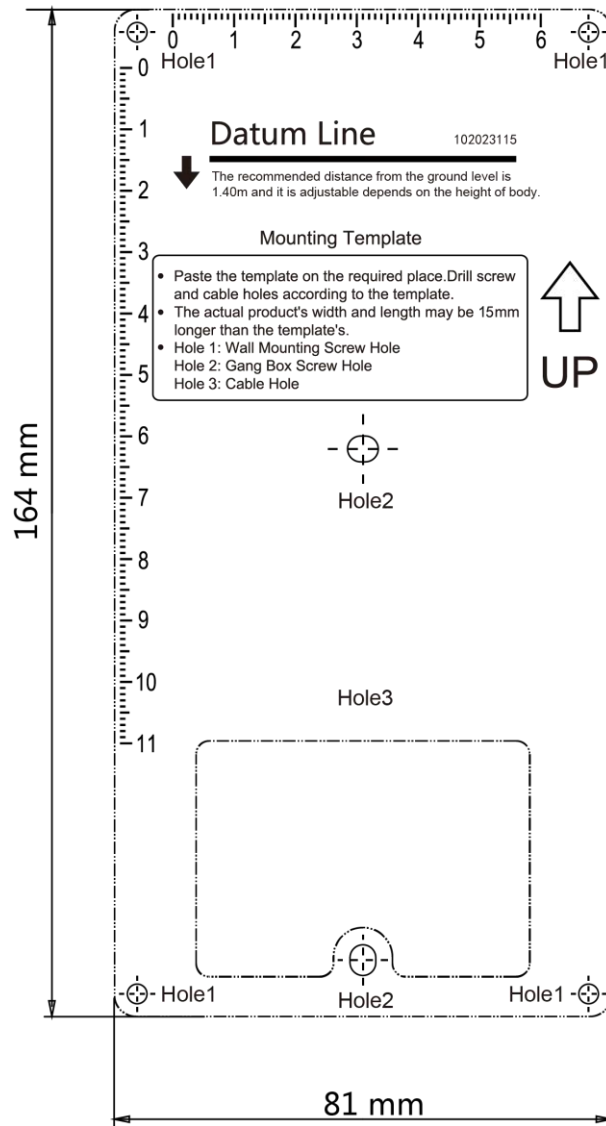
Figure 3-8 Mounting Template
