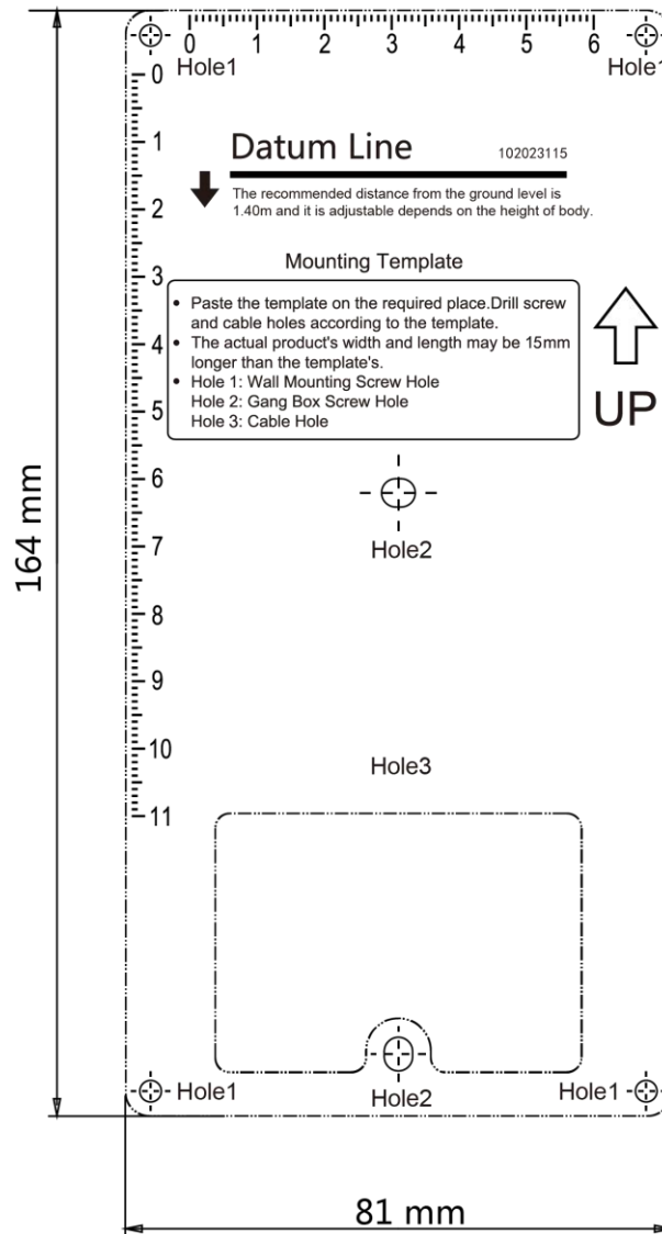
Figure 3-2 Mounting Template
