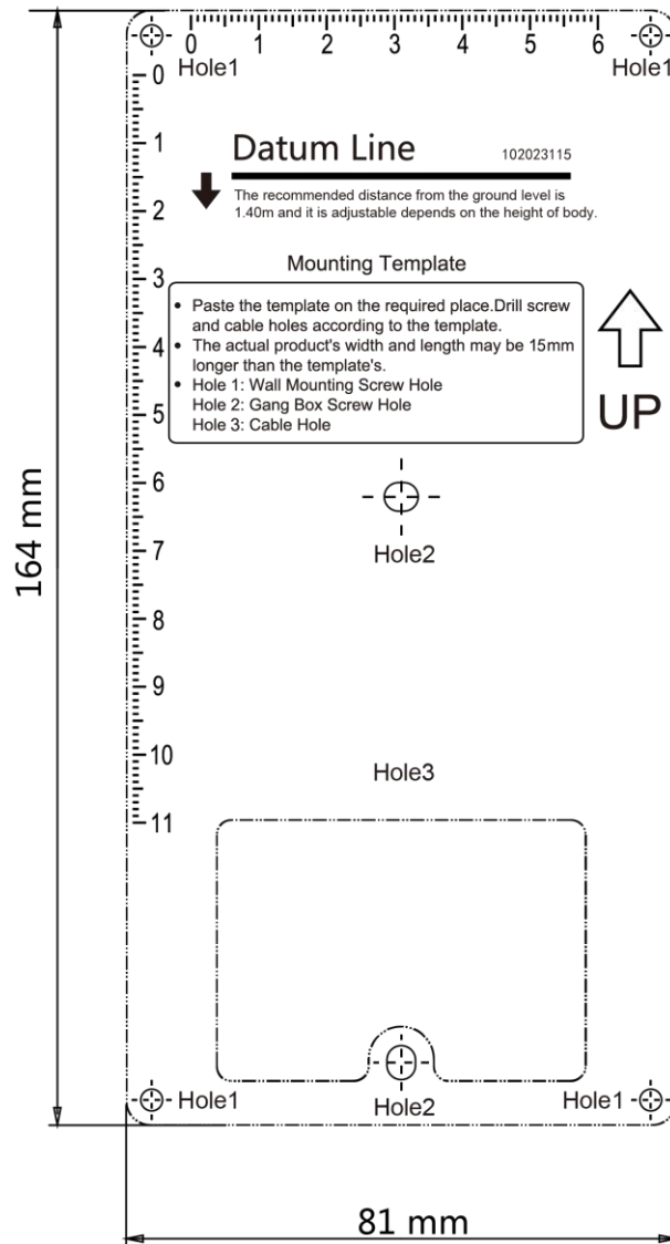
Figure 3-4 Mounting Template
