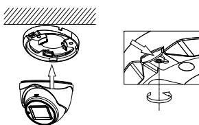
Figure 2-11 Install the Turret Camera
