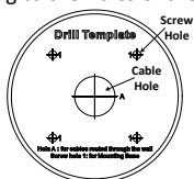
Figure 2-13 Drill Template of the Junction Box
