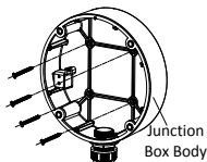
Figure 2-15 Secure the Junction Box's Body on Ceiling
