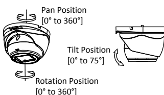
Figure 2-12 3-axis Adjustment
